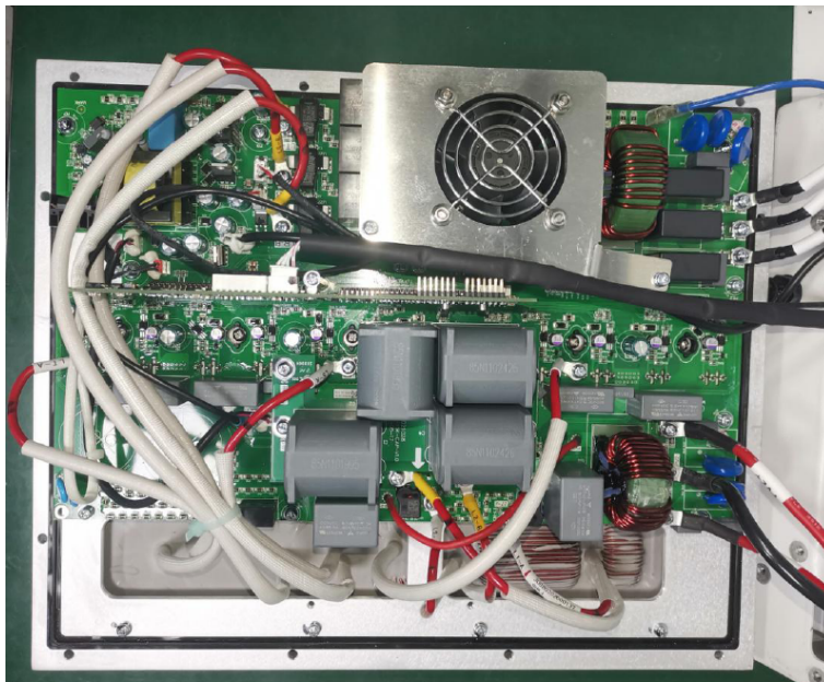
PIC2: Sample Photo, after IP6X test, no dust inside
